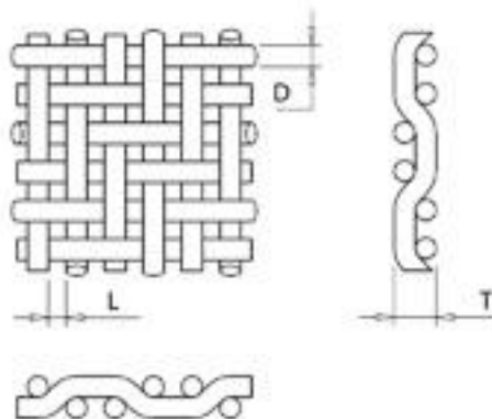
Twilled Weave
