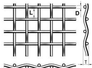
Plain Crimped
