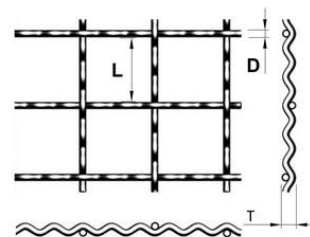
Double Crimped
