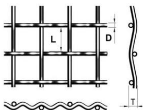
Single Crimped
