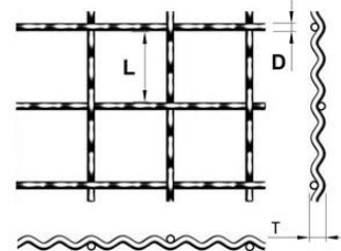
Double Crimped
